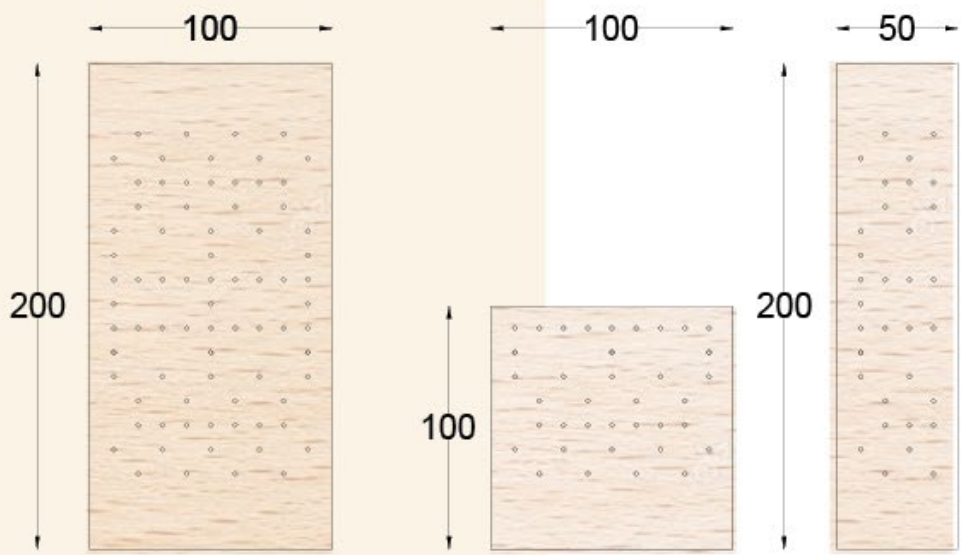
Plan PanWel - 1:20 scale
